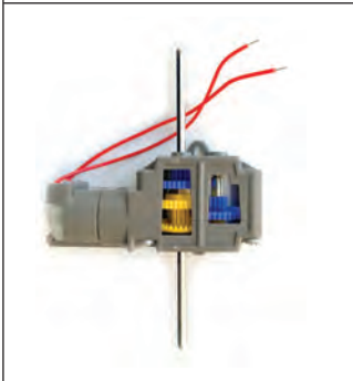
Solar car – Motor and gearbox
